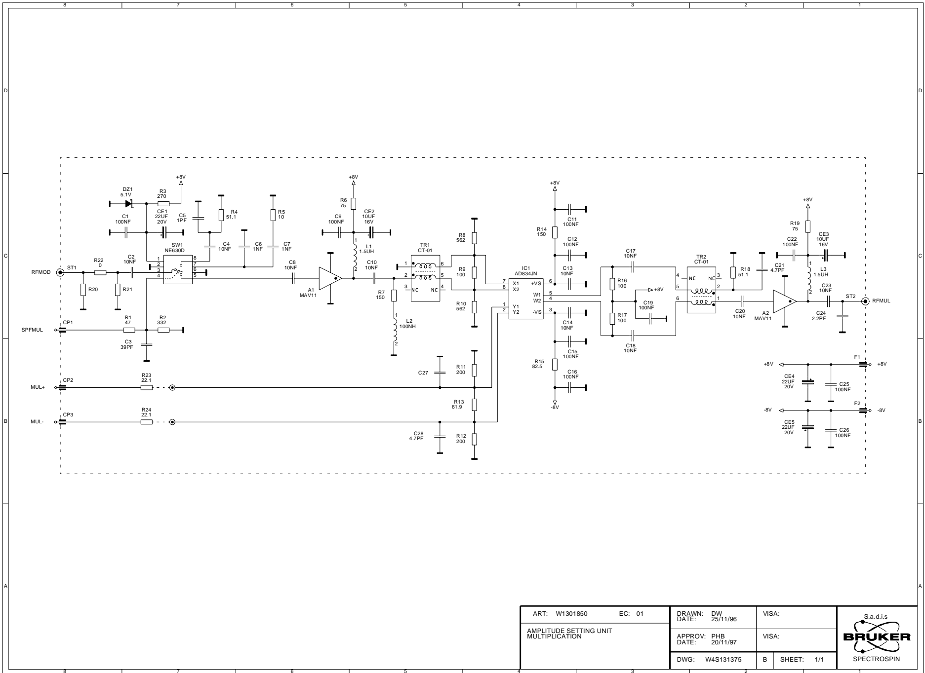
Figure 3.4. Multiplication Schematic
