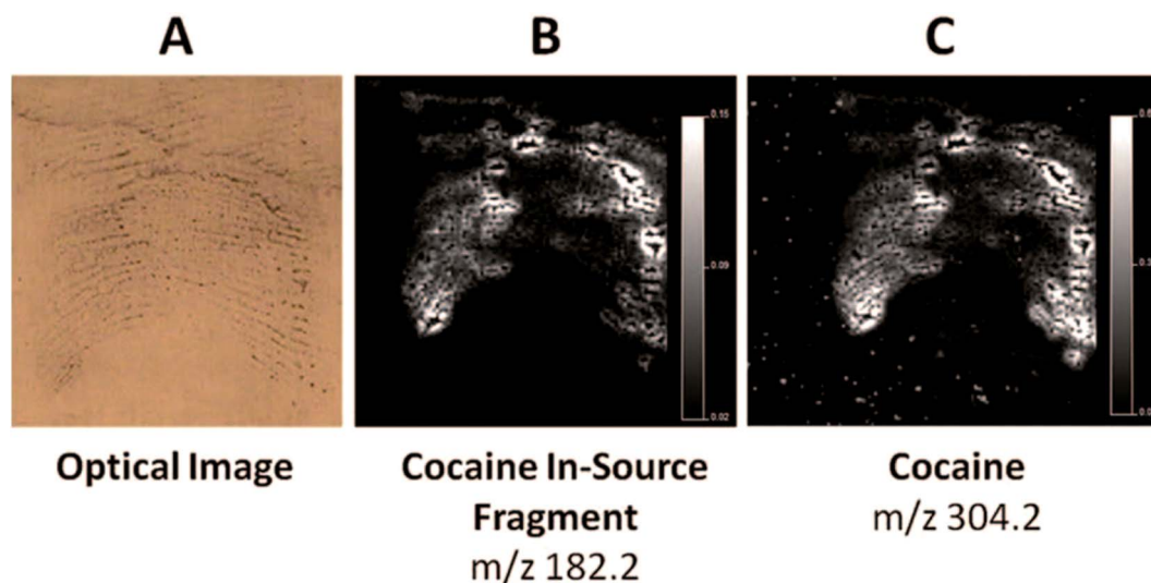
Fig. 5 MALDI-MSI analysis of Print 4, lifted from an interior window frame. (A) Optical image of the print after enhancement with carbon black powder. (B) MALDI-MSI image of the cocaine fragment at m/z 182.2. (C) MALDI-MSI image of protonated cocaine m/z 304.2. (Reproduced as part of open access, Bradshaw et al. 2017, RSC.) 77
