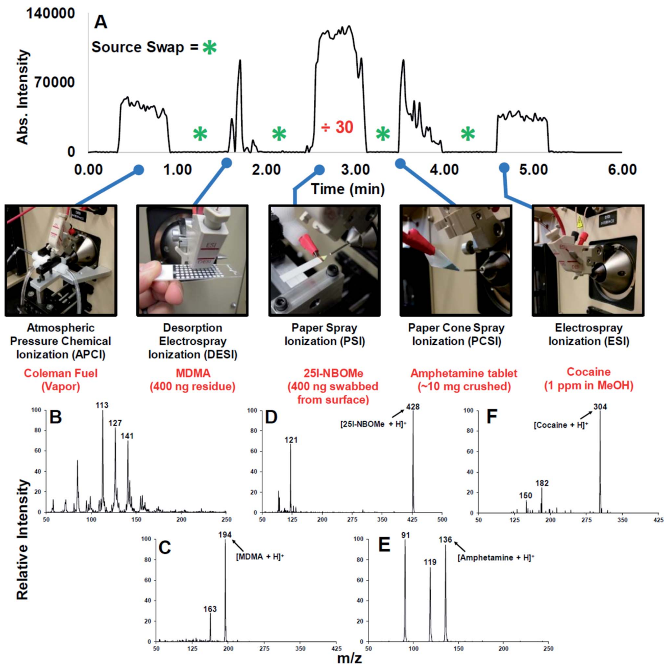
Fig. 12 (A) TIC of entire run (6 minutes), showing 5 discrete source and sample combinations with time required to switch source seen by the signal return to baseline (B) APCI-MS data collected for Coleman Fuel. (C) DESI-MS data collected from MDMA residue. (D) PSI-MS data collected from swabbed 25I-NBOMe residue. (E) PCSI-MS data collected from an amphetamine tablet. (F) ESI-MS data collected from a cocaine extract. (Reproduced with permission, Lawton et al. 2017, ACS.) 28
