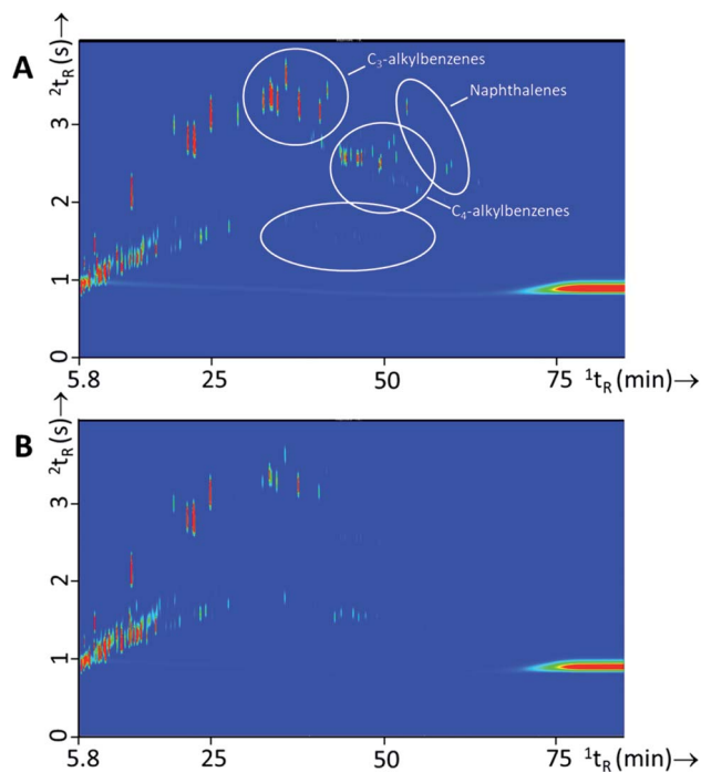
Fig. 3 GC×GC-TOFMS TIC contour plots of two brands of gasoline, (A) Shell (B) BP. White circles highlight differences between the samples. (Reproduced as part of open access, Sampat et al. 2018, MDPI). 44
