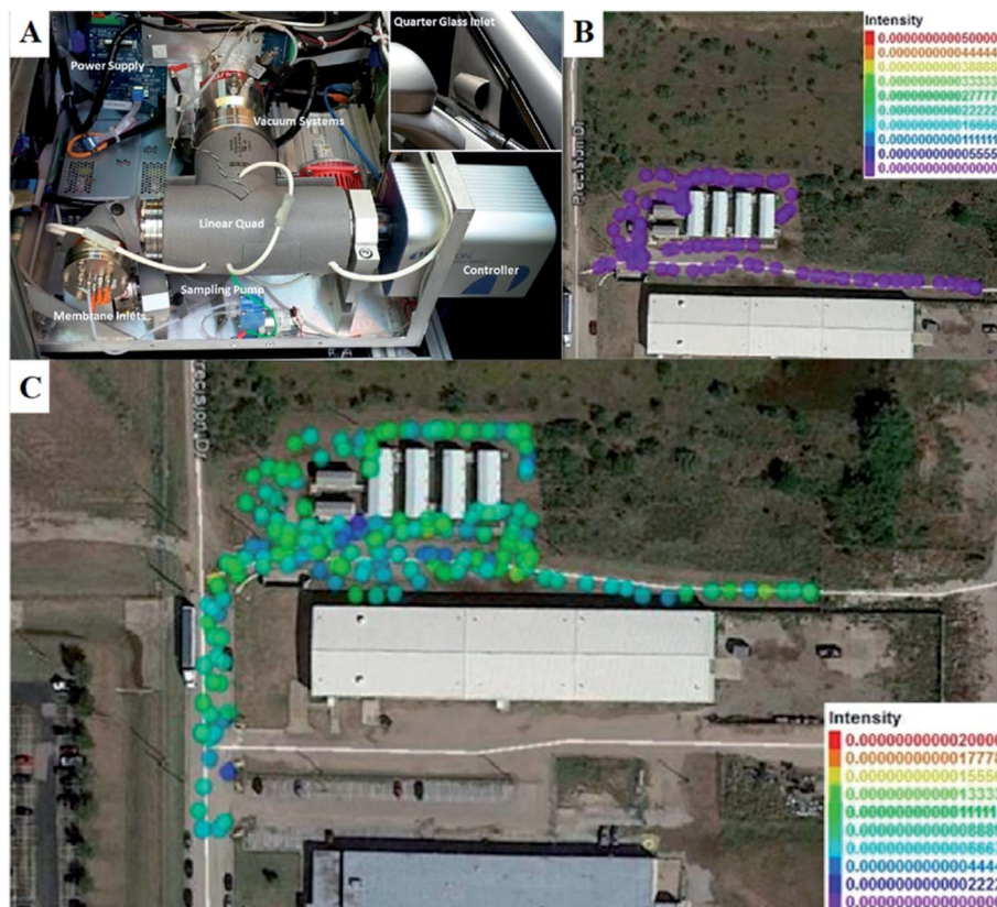
Fig. 11 (A) Portable MIMS system replacing the front passenger seat in vehicle. (B) Baseline MS data before starting reaction, mapped around lab location. (C) MS data obtained from displacement of dibenzylketone, a common impurity, during mock manufacture. (Reproduced with permission, Mach et al. 2015, ACS.) 195
