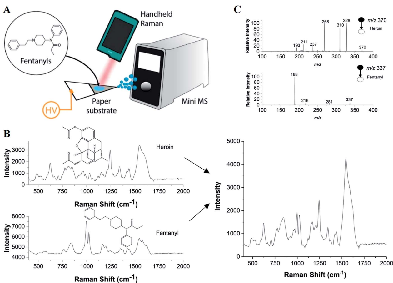
Fig. 14 (A) Depiction of pSERS-MS setup using handheld Raman and miniature MS; nanoparticles are printed on paper substrate to allow for SERS detection, followed by PSI-MS. (B) Raman spectra for morphine and hydromorphone (isobars). (C) CID spectra for morphine and hydromorphone, m/z 286 isolated and fragmented. (Reproduced with permission, Fedick et al. 2017, ACS.) 218 (Reproduced with permission, Fedick et al. 2020, ACS.) 219
