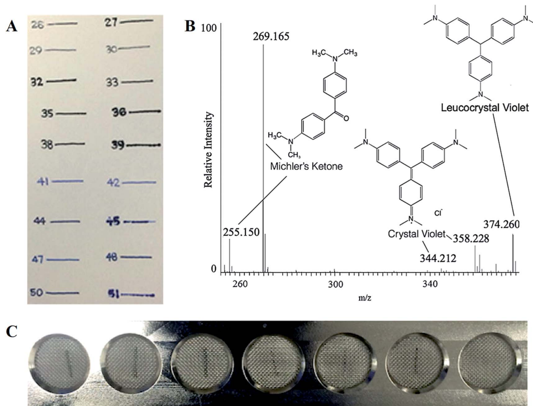
Fig. 9 (A) Ink samples used for analysis. (B) DSA spectrum of degradation peaks of Crystal Violet and Michler's Ketone. (C) Samples aligned via mesh grid in the DSA sample holder. (Reproduced with permission, Nguyen et al. 2018, Elsevier.) 169
