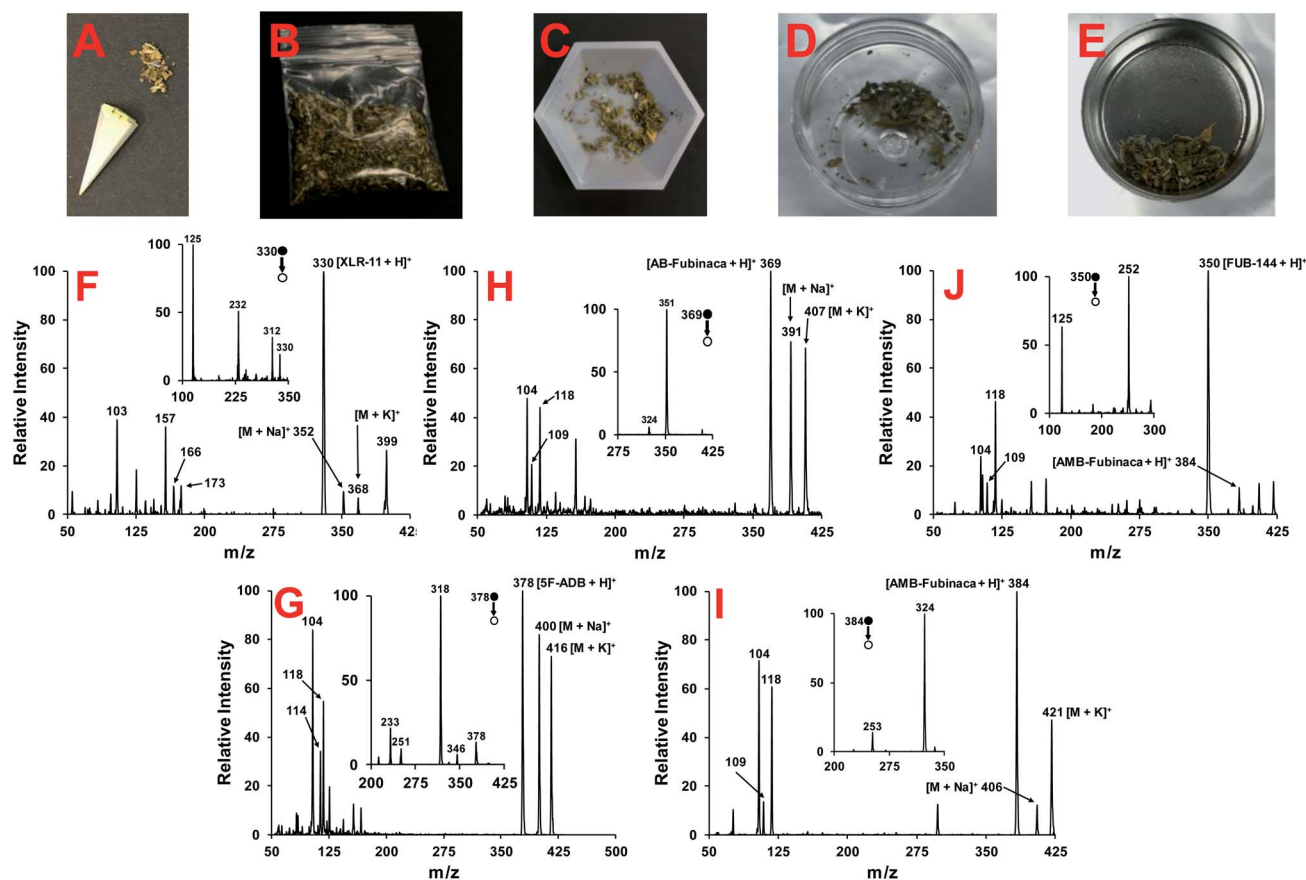
Fig. 13 Synthetic marijuana seizures collected in Central Illinois, including (A) XLR-11, (B) 5F-ADB, (C) AB-Fubinaca, (D) AMB-Fubinaca, and (E) FUB-144, with corresponding FCSI-MS and MS/MS spectra seen in (F)–(I), respectively. The majority of seizures contained one predominant synthetic cannabinoid, however, a few contained multiple illicit chemicals. (Reproduced with permission, Fatigante et al. 2020, ACS.) 216
