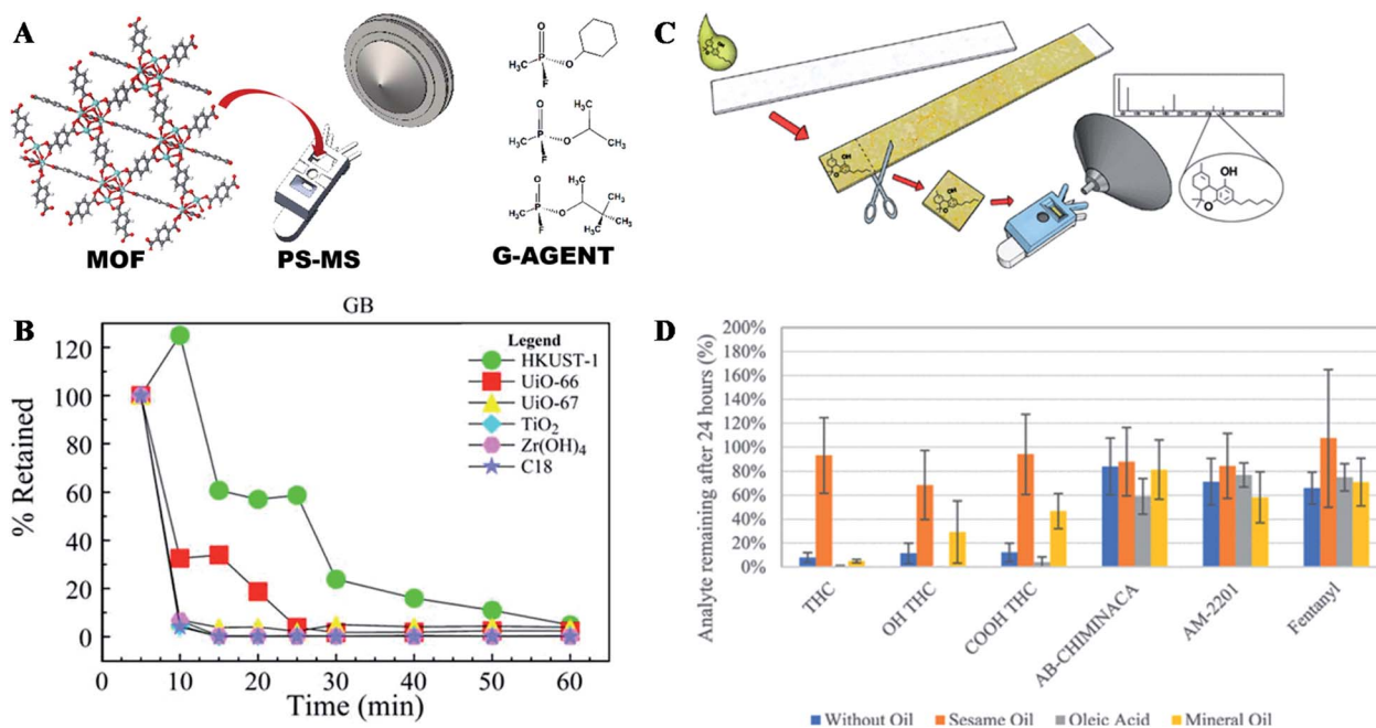
Fig. 8 Modification of paper substrates to improve PSI-MS analysis. (A) Paper substrate modified with MOFs to improve analysis of GB (sarin) CWA. (B) Retention curves over time of G-series CWAs. (C) Sesame oil added to paper substrate to preserve and preconcentrate THC. (D) Comparison of different oils used to preserve analytes. Shown in percent analyte remaining after 24 h vs. 1 h in urine. (Reproduced with permission, Dhummakupt et al. 2018, ACS.) 157 (Reproduced with permission, Bills et al. 2020, ACS.) 158
