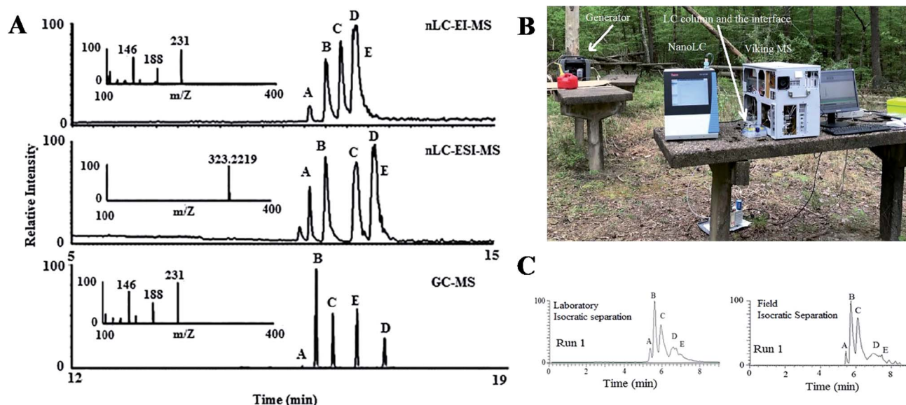
Fig. 4 (A) Comparison of n LC-EI-MS, n LC-ESI-MS, and GC-MS chromatograms. Peaks correspond to heroin (A), acetyl fentanyl (B), fentanyl (C), carfentanyl (D), and butyryl fentanyl (E). Inset shows mass spectra of peak B. (B) Picture of the n LC-EI-MS system in the field. (C) Comparison of isocratic separation chromatograms in the laboratory and in the field. (Reproduced with permission, Abonamah et al. 2019, Elsevier.) 62
